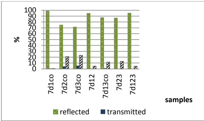
Fig. 10. SE (%) of double jersey samples ( g = E7 ) with metallized threads parallel to polarization plane of the electromagnetic wave 1.161 GHz.
