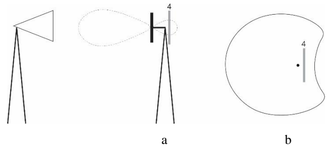
Fig. 9. Radiation pattern (electric filed intensity) of dipole in vertical polarization, with sample: a – cross section side view and b – from above.
